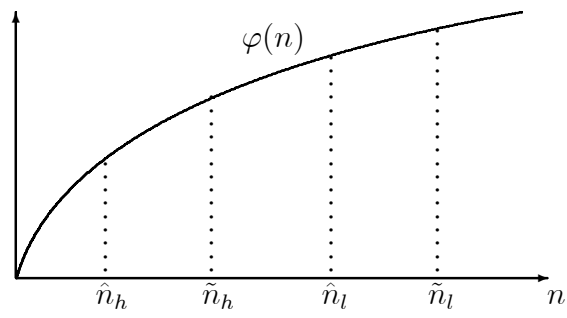
Figure 2: Voters' utility
