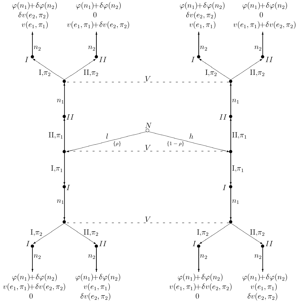
Figure 1: The extensive form game
